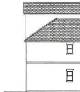
Side Elevation 1:100
